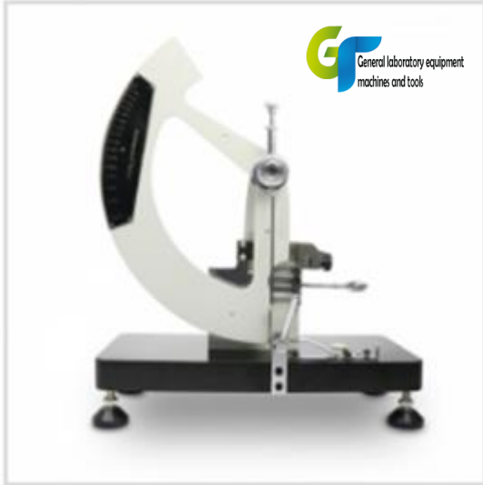
Elmendorf Tearing Tester GT-C10
